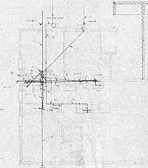
PLUMBING PLAN - UNIT CR
