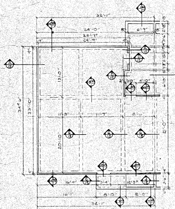
FOUNDATION PLAN - UNIT CR
