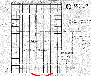
ROOF FRAMING PLAN - UNIT CR
