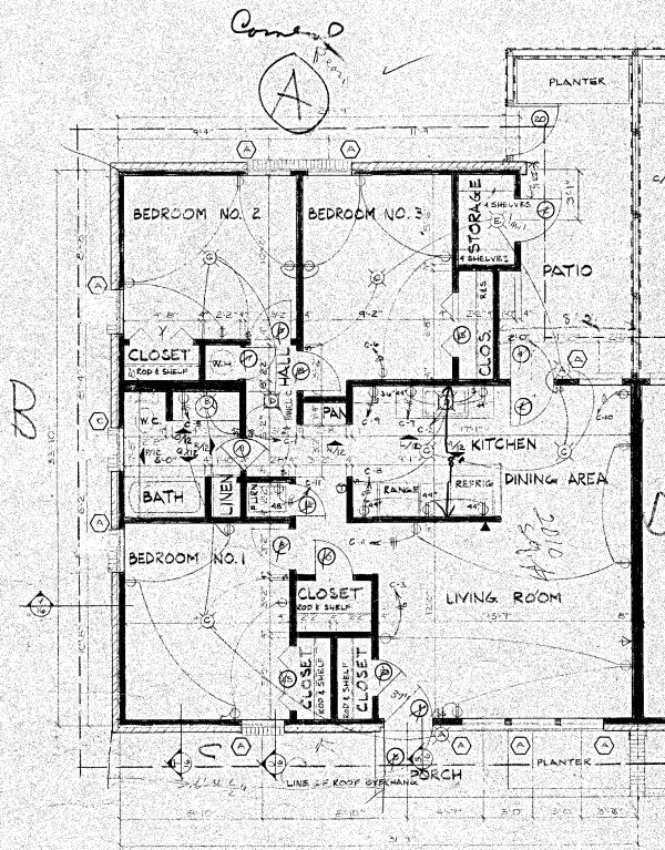
FLOOR PLAN - UNIT CR
