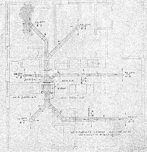
HEATING PLAN - UNIT CR
